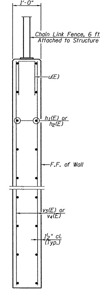
SECTION THRU CONCRETE FACING (Looking East)
