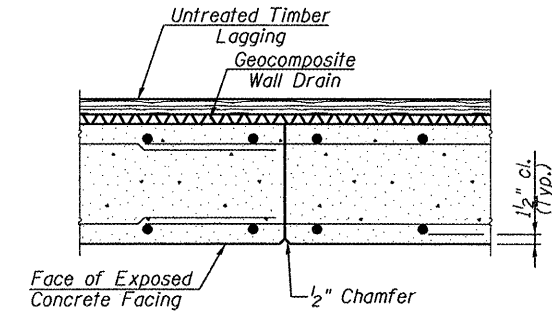
WALL CONSTRUCTION JOINT
