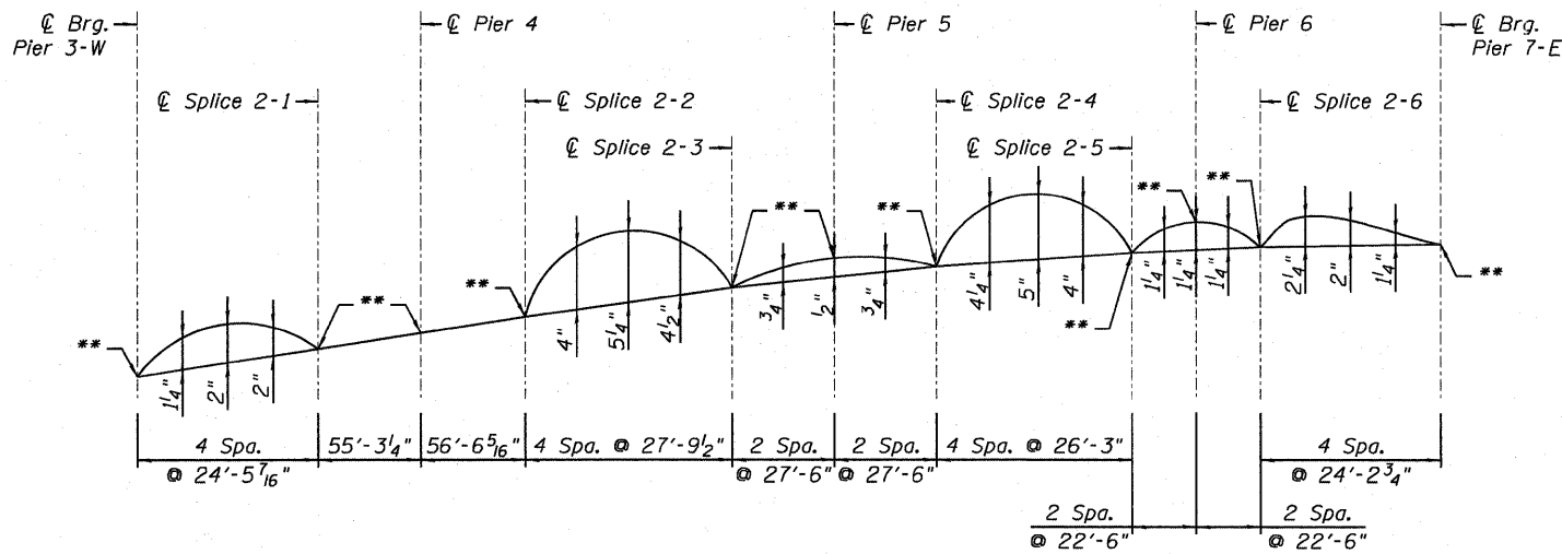
CAMBER DIAGRAM - S.N. 082-0325 - UNIT 2 (GIRDER 1A)
