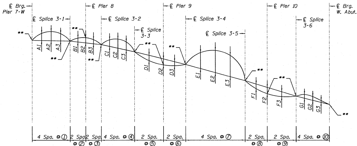
CAMBER DIAGRAM - S.N. 082-0325 - UNIT 3 (GIRDERS 1B THRU 7B)
