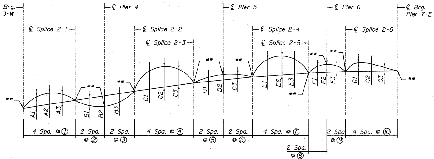
CAMBER DIAGRAM - S.N. 082-0325 - UNIT 2 (GIRDERS 2A THRU 6A)
