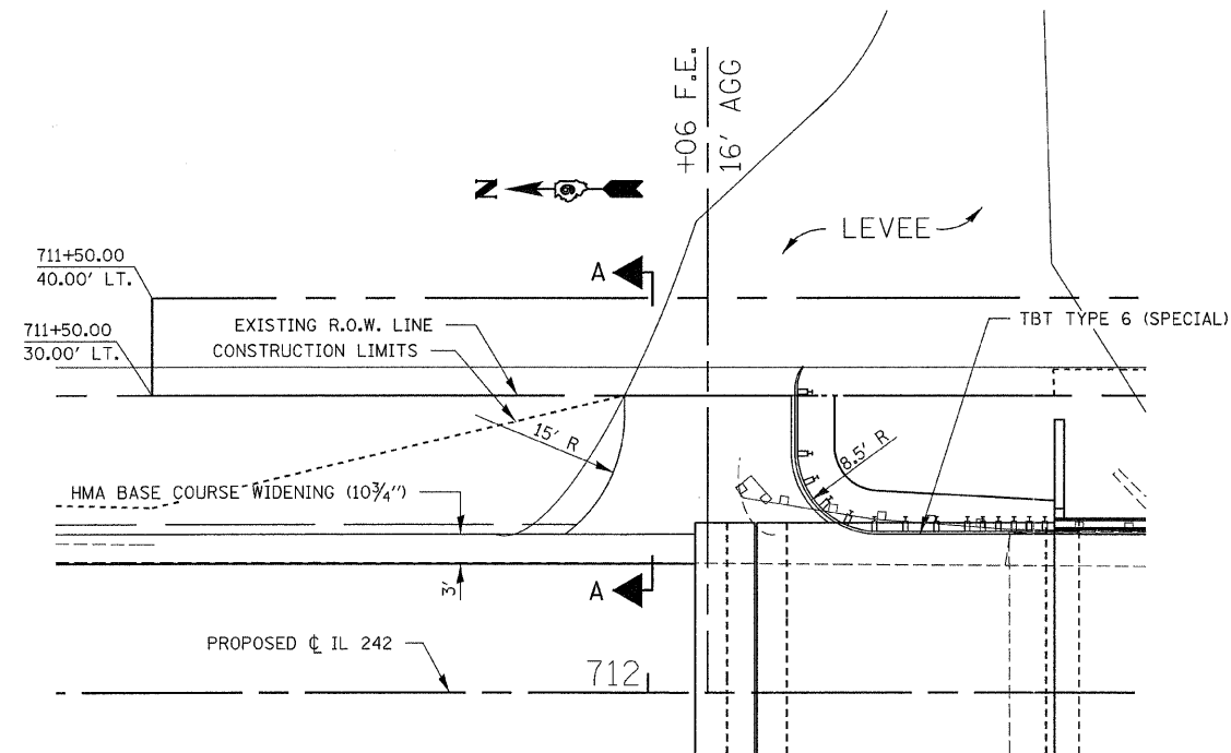
ENTRANCE AND GUARDRAIL DETAIL
