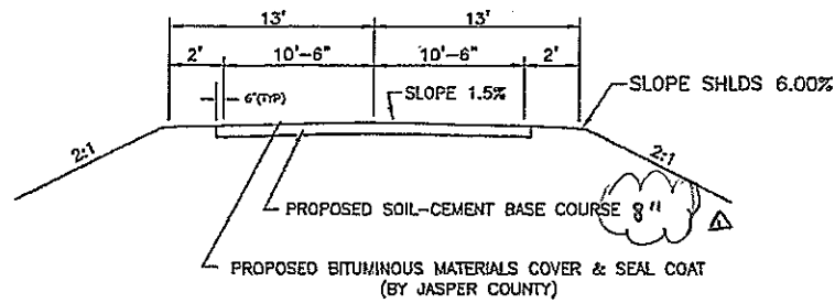
TYPICAL CROSS SECTION OF PROPOSED ROADWAY
