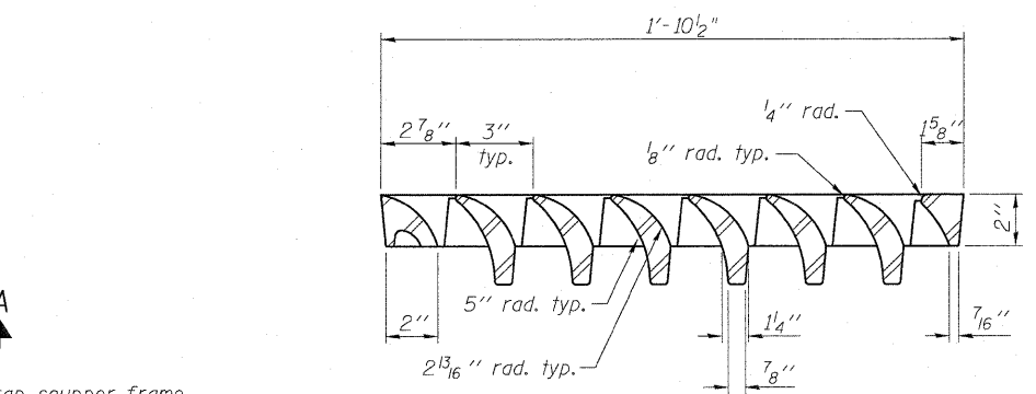
VANE GRATE DETAIL
