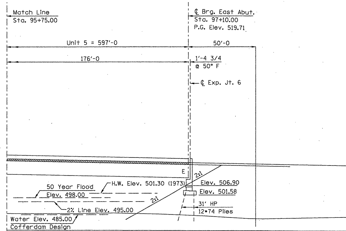
LONGITUDINAL SECTION ALONG U.S. 136
