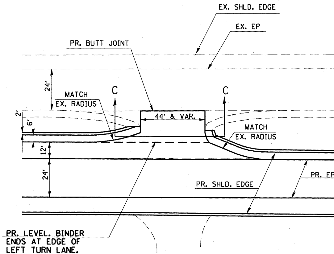
DETAIL FOR MEDIAN CROSSOVER WHERE LEFT TURN LANE IS PRESENT WEST OF IL 166 INTERSECTION (SEE TYPICAL SECTION, SHT. 10)
