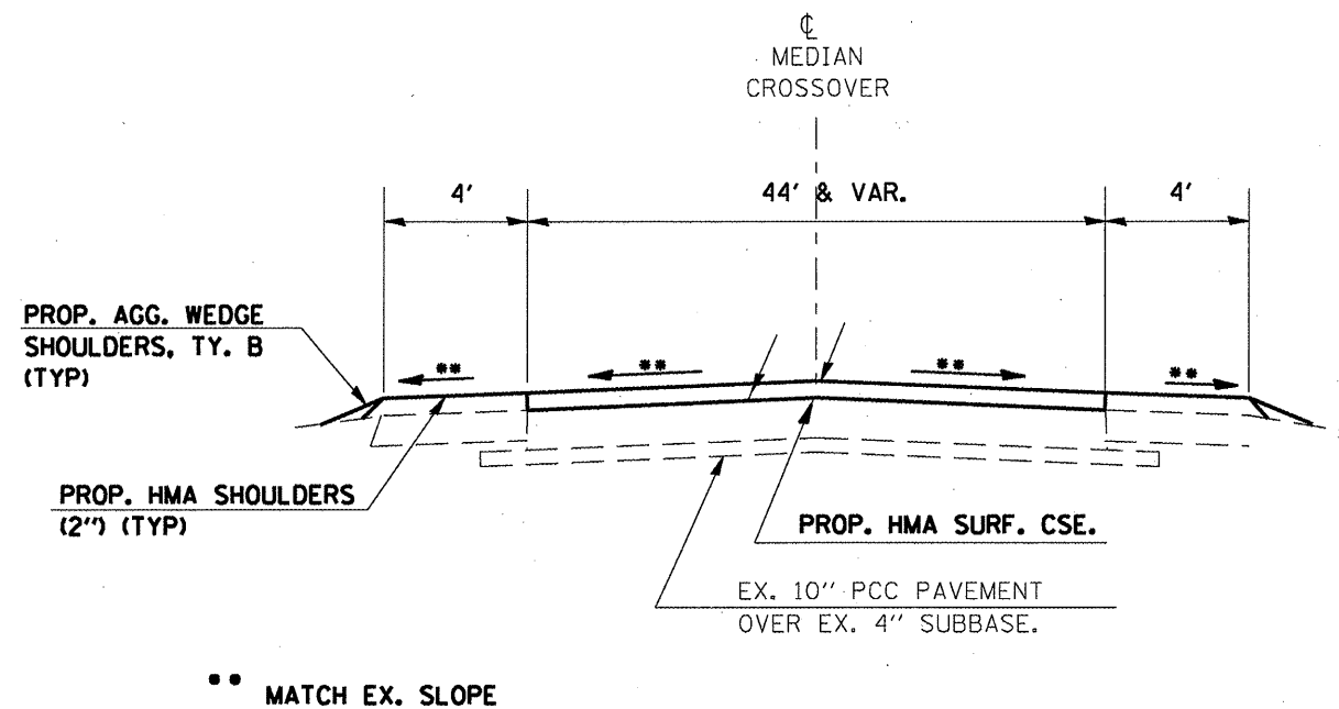
SECTION C - C TYPICAL FOR MEDIAN CROSSOVER
