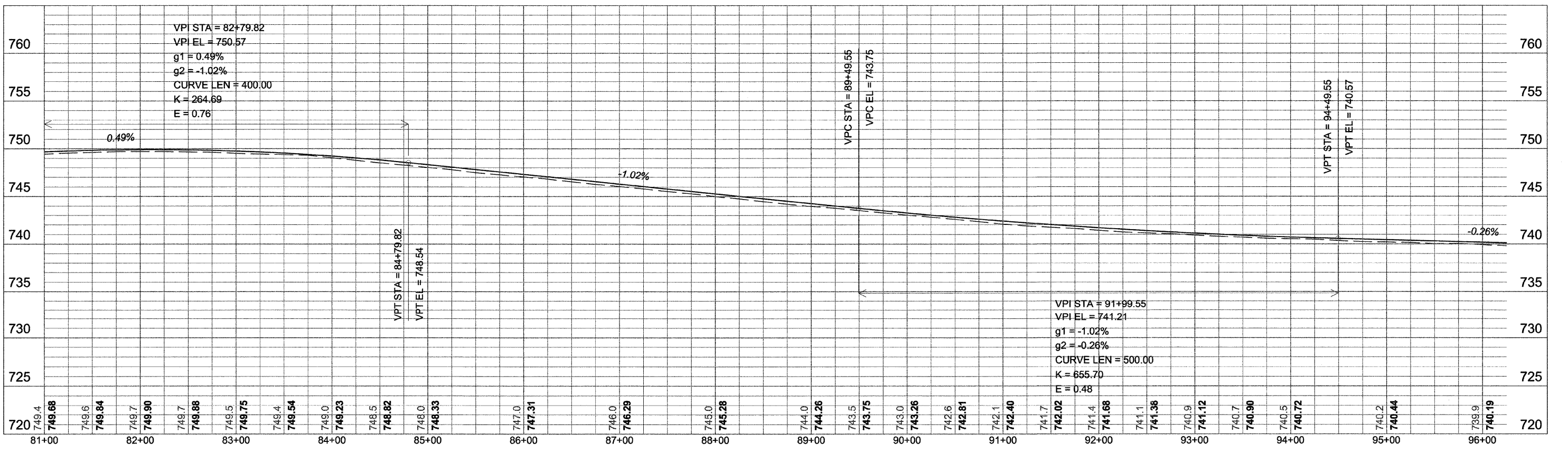
PLAN & PROFILE - HONONEGAH RD
