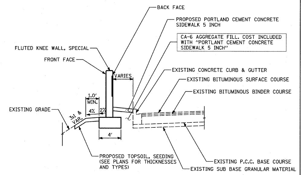
FLUTED KNEE WALL TYPICAL SECTION AT SIDEWALK
