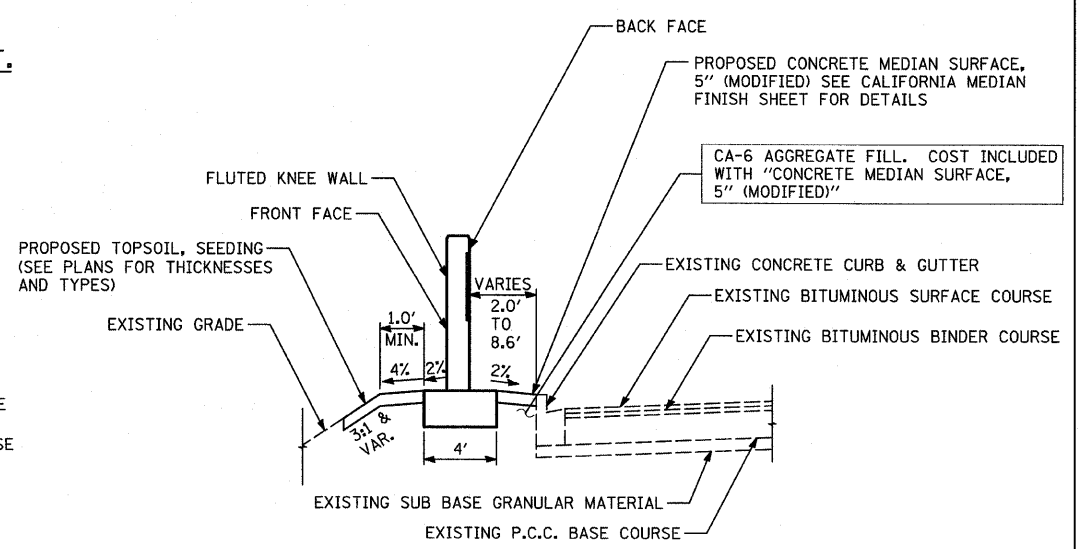
KNEE WALL DETAIL 6
