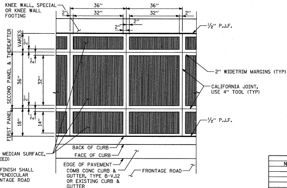
DETAIL "A": COORDINATE WITH CONC. MED. SURFACE, 5" (MODIFIED) "C" CALIFORNIA FINISH
