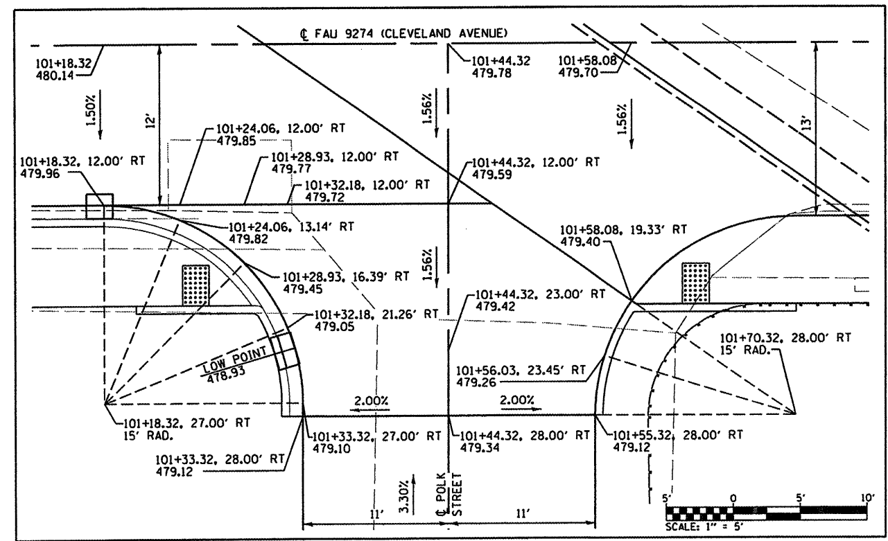
INTERSECTION DETAIL - POLK STREET
