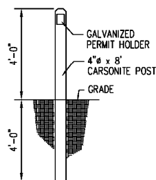
2 C3-5 SCALE: ? = 1'-0" TYPICAL RV SITE MARKER & PERMIT POST DETAIL
