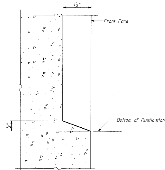
DETAIL B
