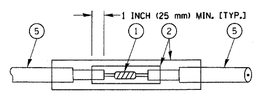
DETAIL "A" LOOP-TO-LOOP SPLICE
