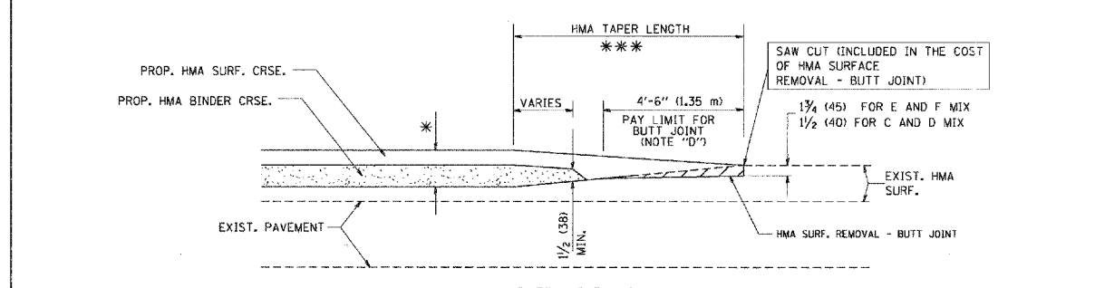
OPTION 2 TYPICAL TEMPORARY RAMP
