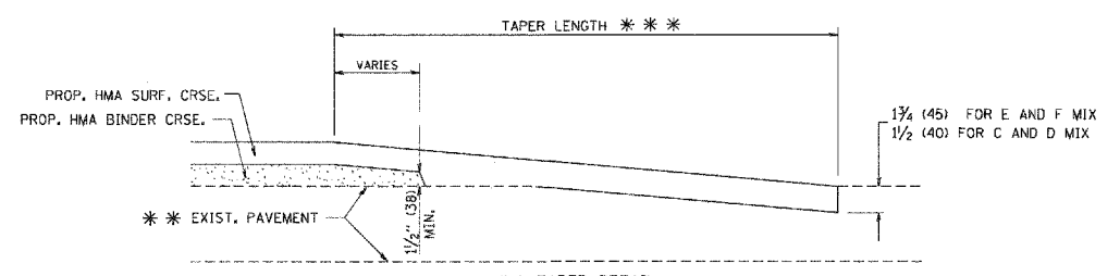
HMA TAPER DETAIL
