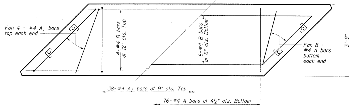
SLAB REINFORCEMENT
