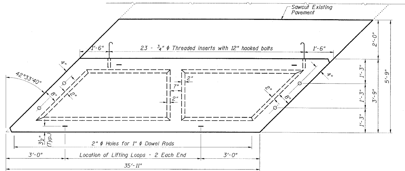
PARTIAL PLAN OF APPROACH
