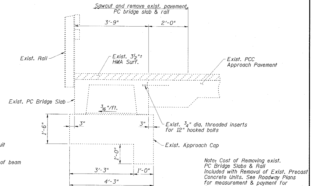
EXISTING CROSS SECTION
