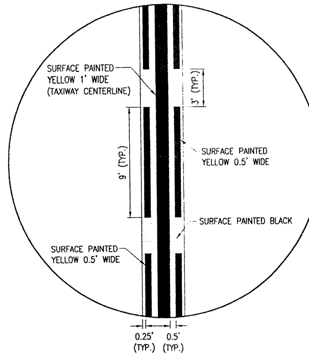
ENHANCED TAXIWAY MARKING DETAIL "NOT TO SCALE"
