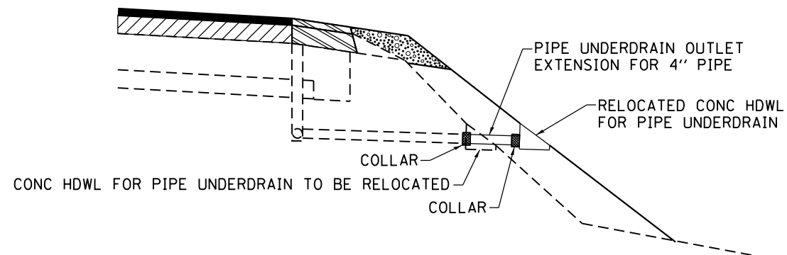
PIPE UNDERDRAIN OUTLET EXTENSION SPECIAL
