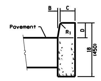
BARRIER CURB
