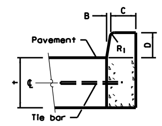
BARRIER CURB
