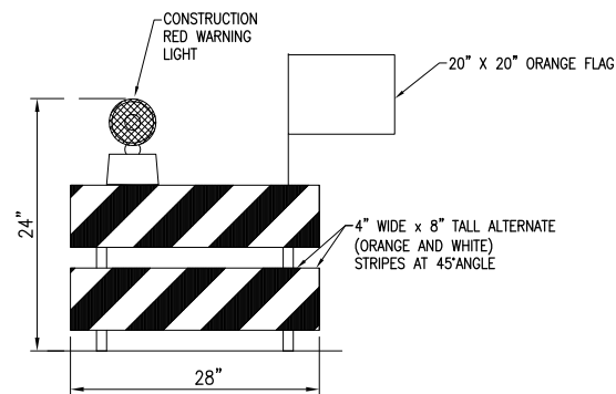
MODIFIED TYPE II BARRICADE NOT TO SCALE
