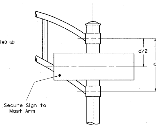
DUAL ARM
