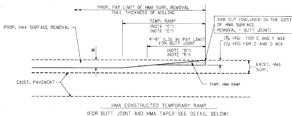
OPTION 2 TYPICAL TEMPORARY RAMP
