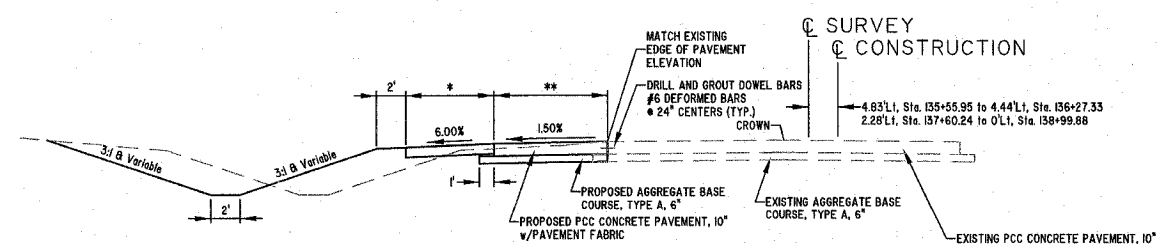
TYPICAL SECTION - FAYETTE AVENUE (PROPOSED) STA. 135+55.95 TO STA. 136+27.33 STA. 137+60.24 TO STA. 39+75.06 STATION EQUATION: CONSTRUCTION STA. 138+99.88 (B)+ SURVEY STA. 39+00.00 (A)+
