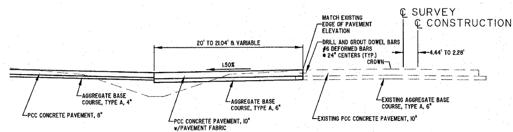
TYPICAL SECTION - FAYETTE AVENUE (PROPOSED) STA. 136+27.33 TO STA. 137+60.24
