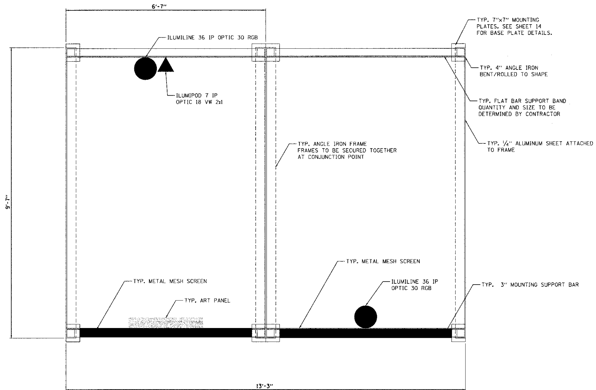
PLAN
