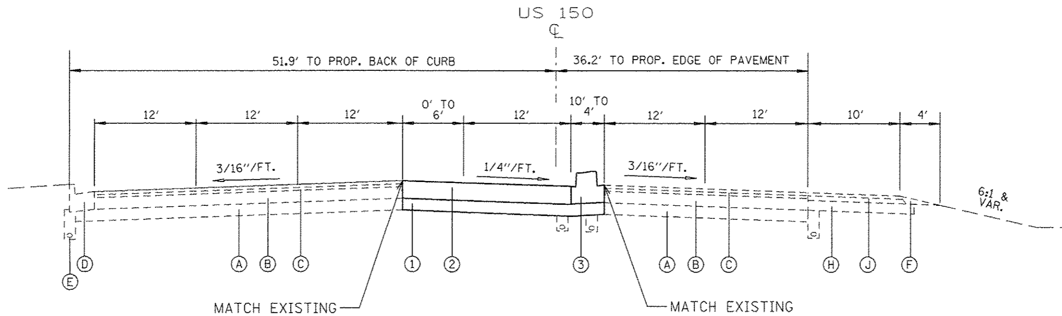
PROPOSED TYPICAL SECTION (US. RTE. 150) STA. 492+32 TO STA. 495+07.5
