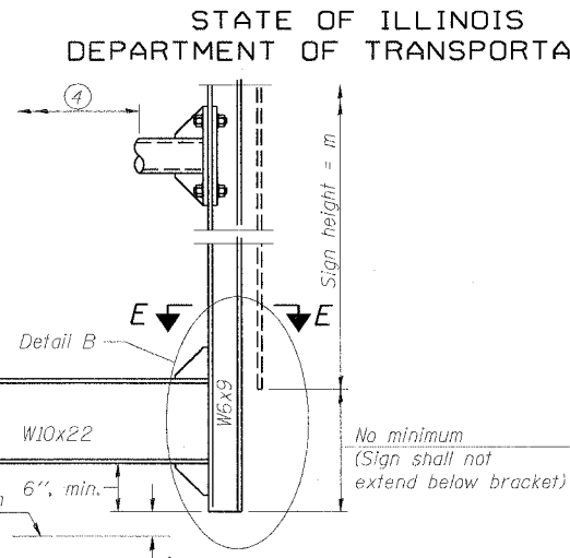
SECTION A-A Alternate with no lights or walkways ④ For attachment details of 3/2" pipe and W10x22, see other sections as applicable.
