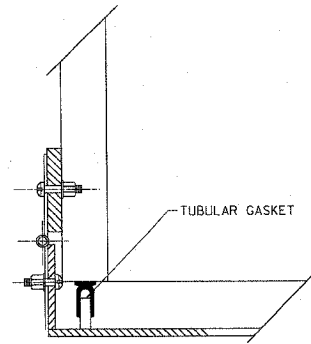
HINGE DETAIL
