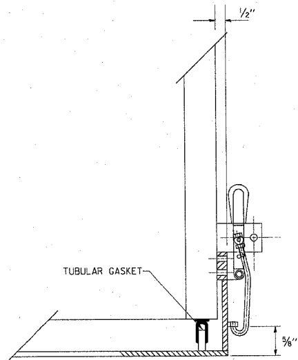
LATCH DETAIL
