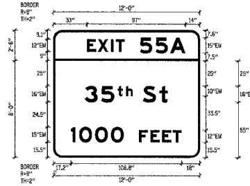
SIGN DETAIL 1:50
