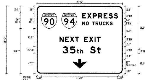
SIGN DETAIL 1:50
