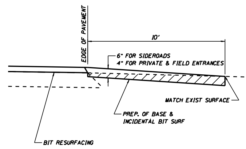
SECTION B-B FOR OIL & CHIP FE & PE, BIT FE AND OIL & CHIP SIDEROAD
