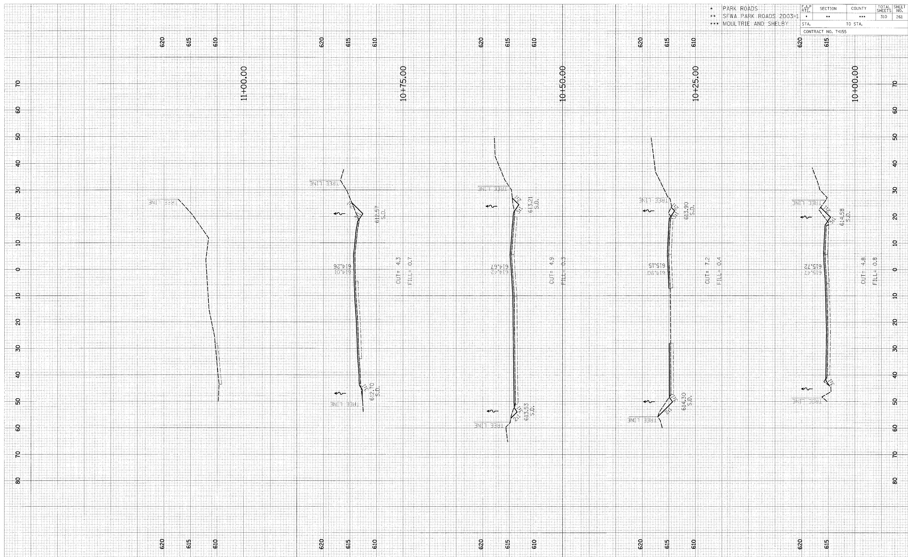
CROSS SECTION, KASKASKIA, TR 142 TO PARKING LOT 64 AND TURN AROUND NO. 1 STA 10+00.00 TO STA 11+00.00
