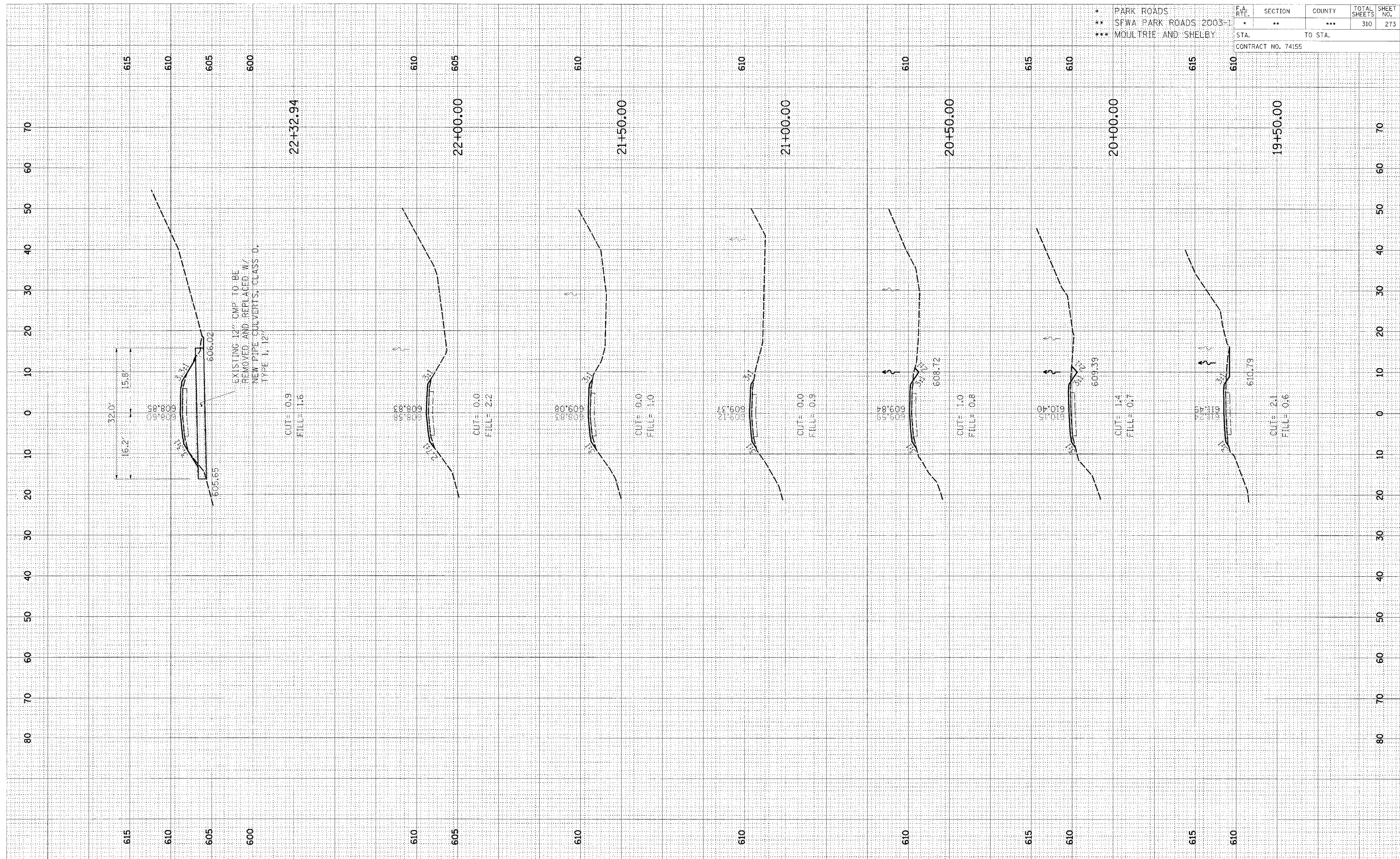
CROSS SECTION, KASKASKIA, PARK ROAD TO PARKING LOT 67, STA 19+50.00 TO STA 22+32.94
