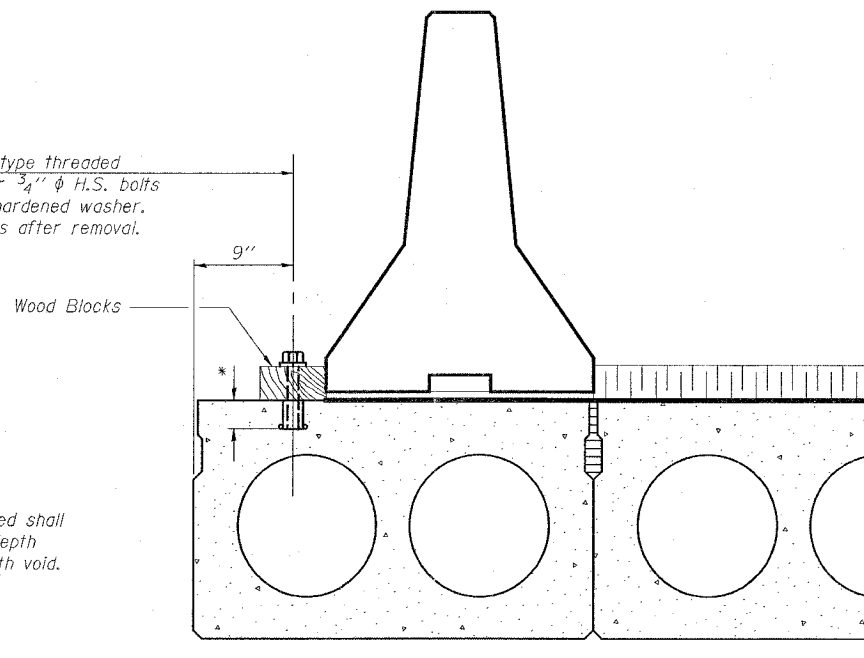
DETAIL I
