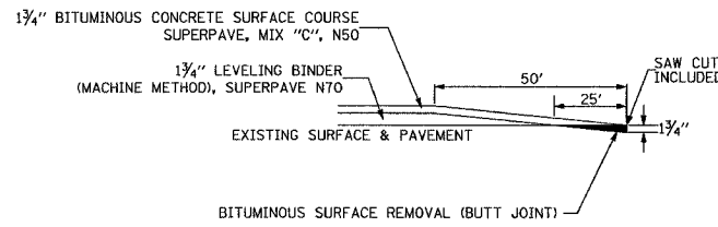
BUTT JOINT DETAIL STA 1+11.9 TO STA 1+61.9
