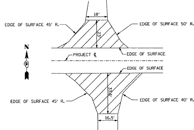
DETAIL OF INTERSECTION LT. STA. 102+50 & RT. STA. 102+58
