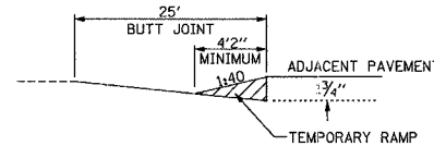
TEMPORARY RAMP DETAIL STA 1+57.73 TO STA 1+61.9
