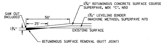
BUTT JOINT DETAIL STA 1+11.9 TO STA 1+61.9
