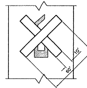
CLOSED RUNWAY MARKER DETAIL
