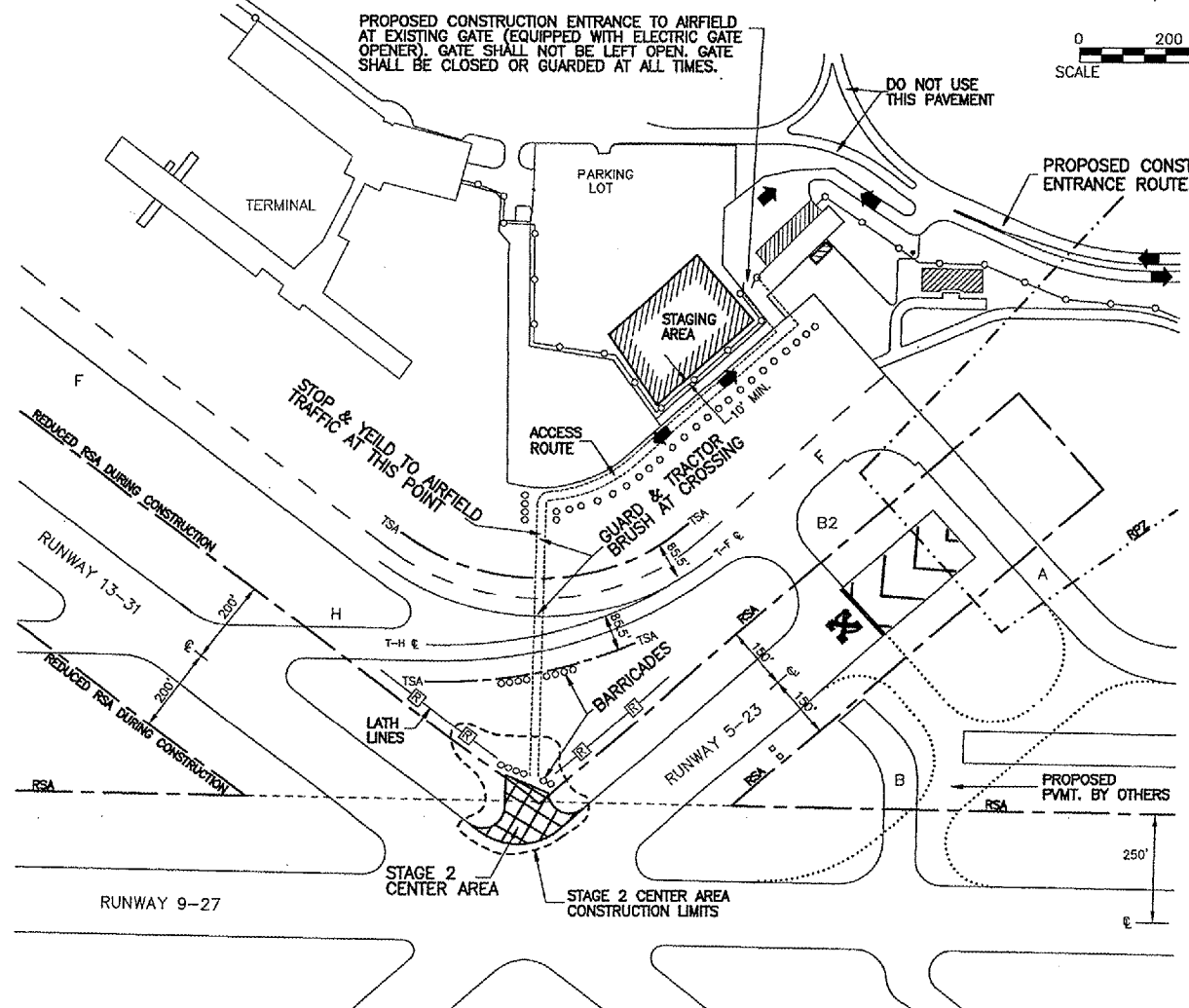
STAGE 2 CENTER AREA BARRICADES, LATH LINES, AND CONSTRUCTION OPERATION LIMITS
