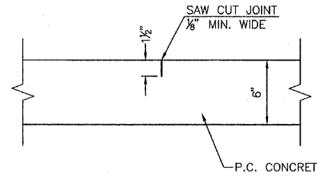
DETAIL OF SAWED CONTRACTION JOINT
