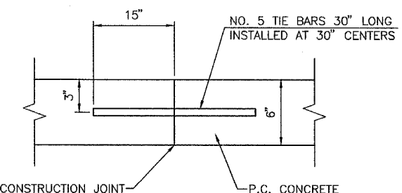
DETAIL OF TIED CONSTRUCTION JOINT
