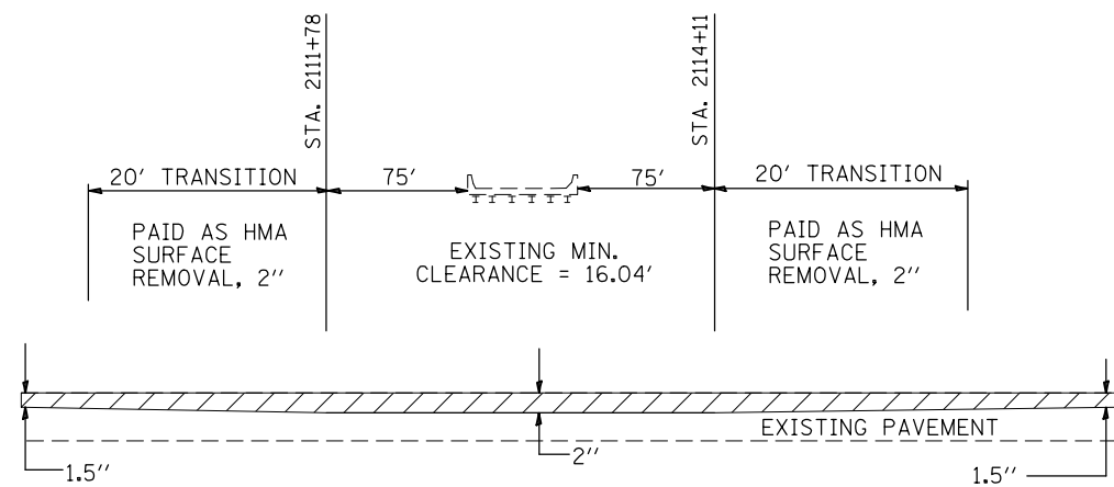
MILLING TRANSITION DETAIL E.B. LANES UNDER S.N. 095-0038 (IL-177)
