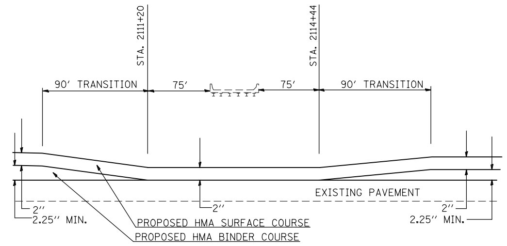
PAVING TRANSITION DETAIL W.B. LANES UNDER S.N. 095-0038 (IL-177)
