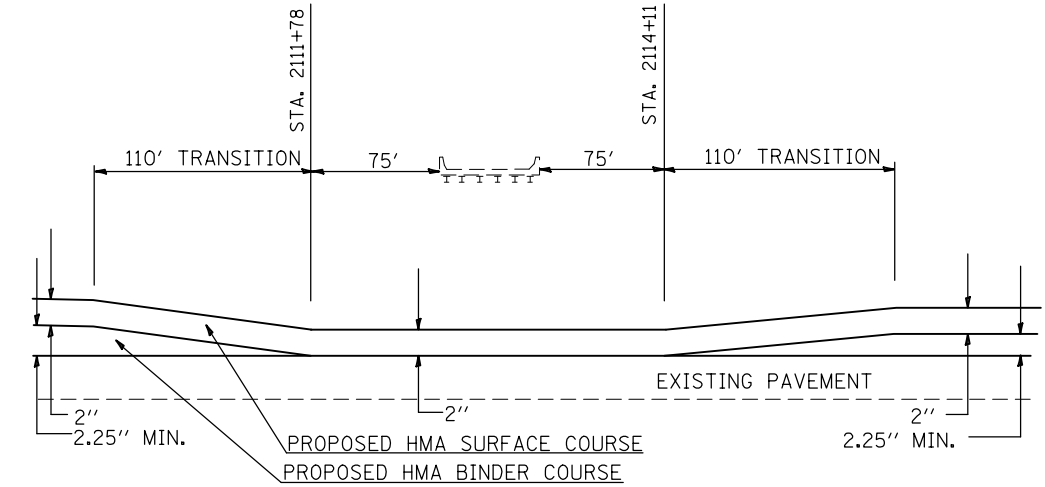
PAVING TRANSITION DETAIL E.B. LANES UNDER S.N. 095-0038 (IL-177)
