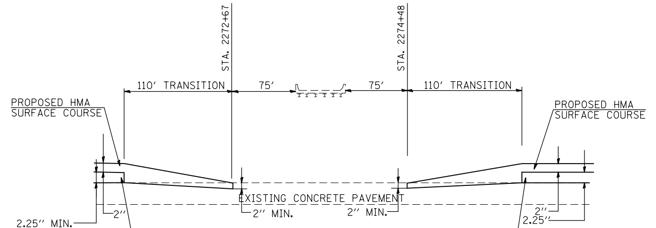
PAVING TRANSITION DETAIL E.B. LANES UNDER S.N. 095-0036 (CH-4)
