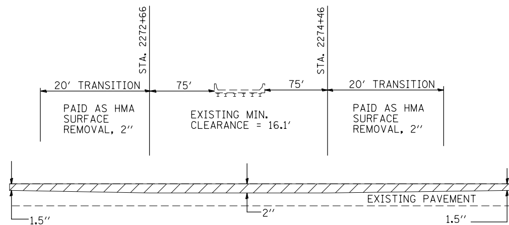
MILLING TRANSITION DETAIL W.B. LANES UNDER S.N. 095-0036 (CH-4)
