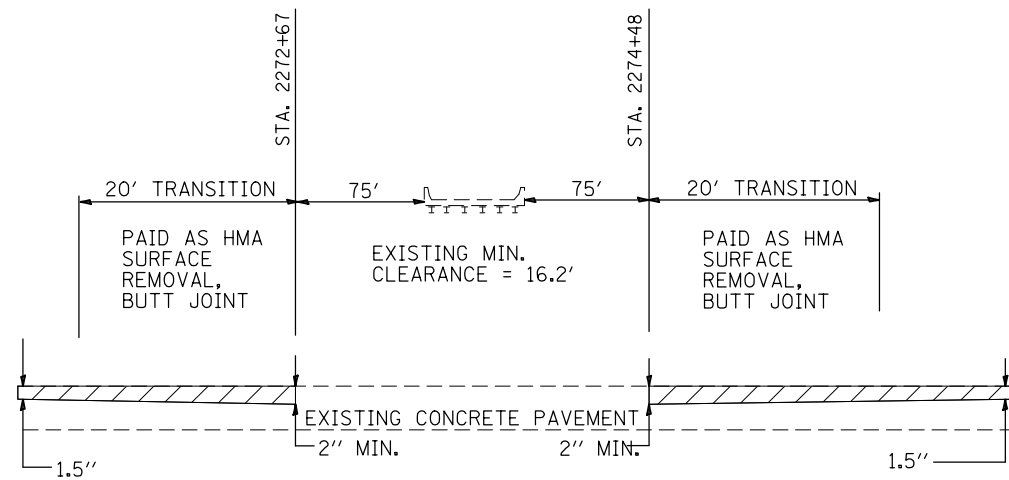
MILLING TRANSITION DETAIL E.B. LANES UNDER S.N. 095-0036 (CH-4)
