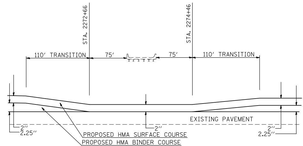
PAVING TRANSITION DETAIL W.B. LANES UNDER S.N. 095-0036 (CH-4)
