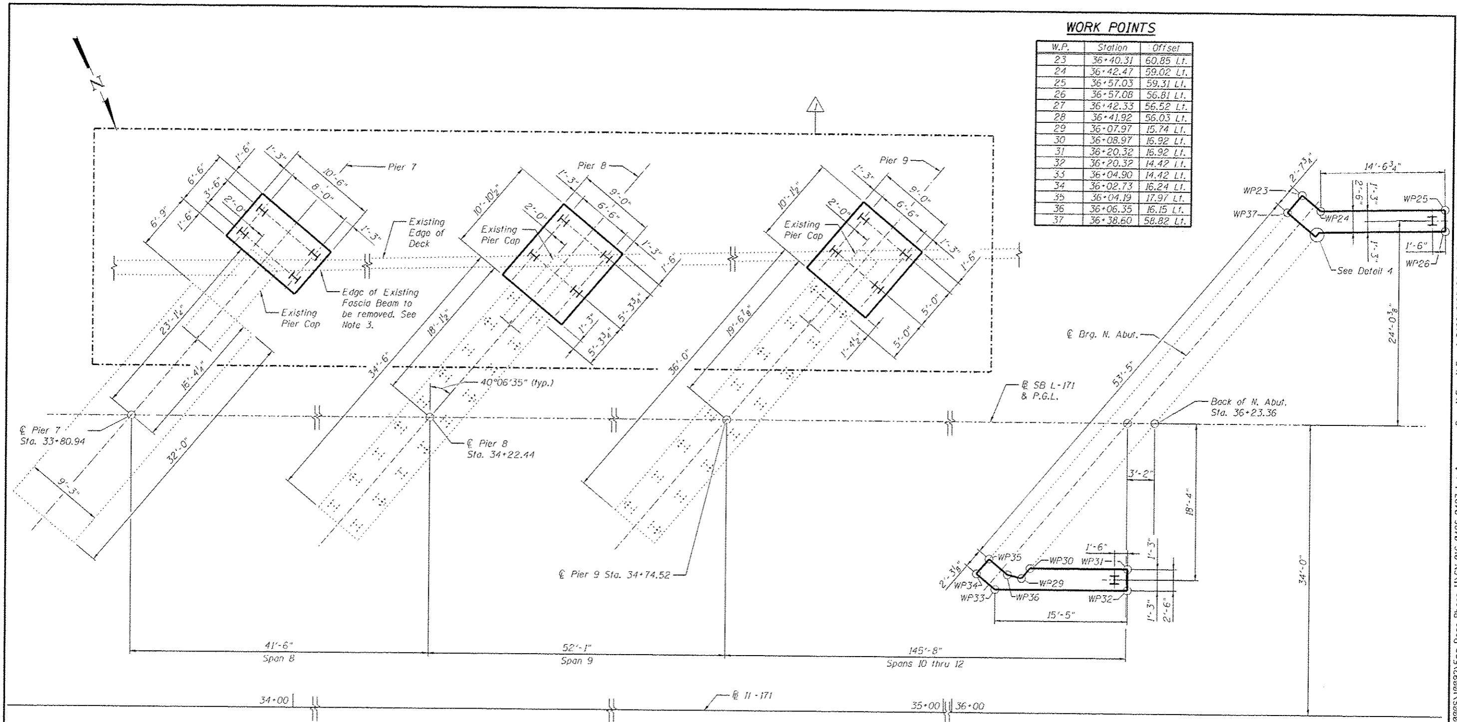
PLAN - FOUNDATION LAYOUT
