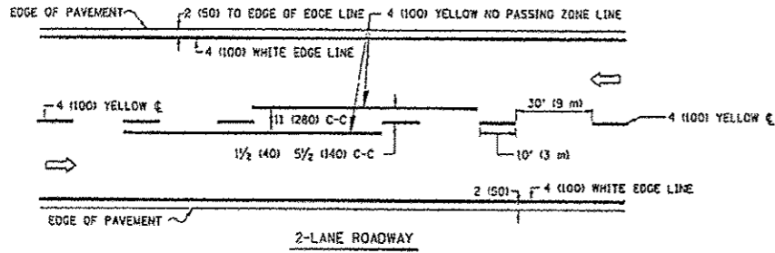
2-LANE ROADWAY
