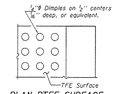
PLAN-PTFE SURFACE
