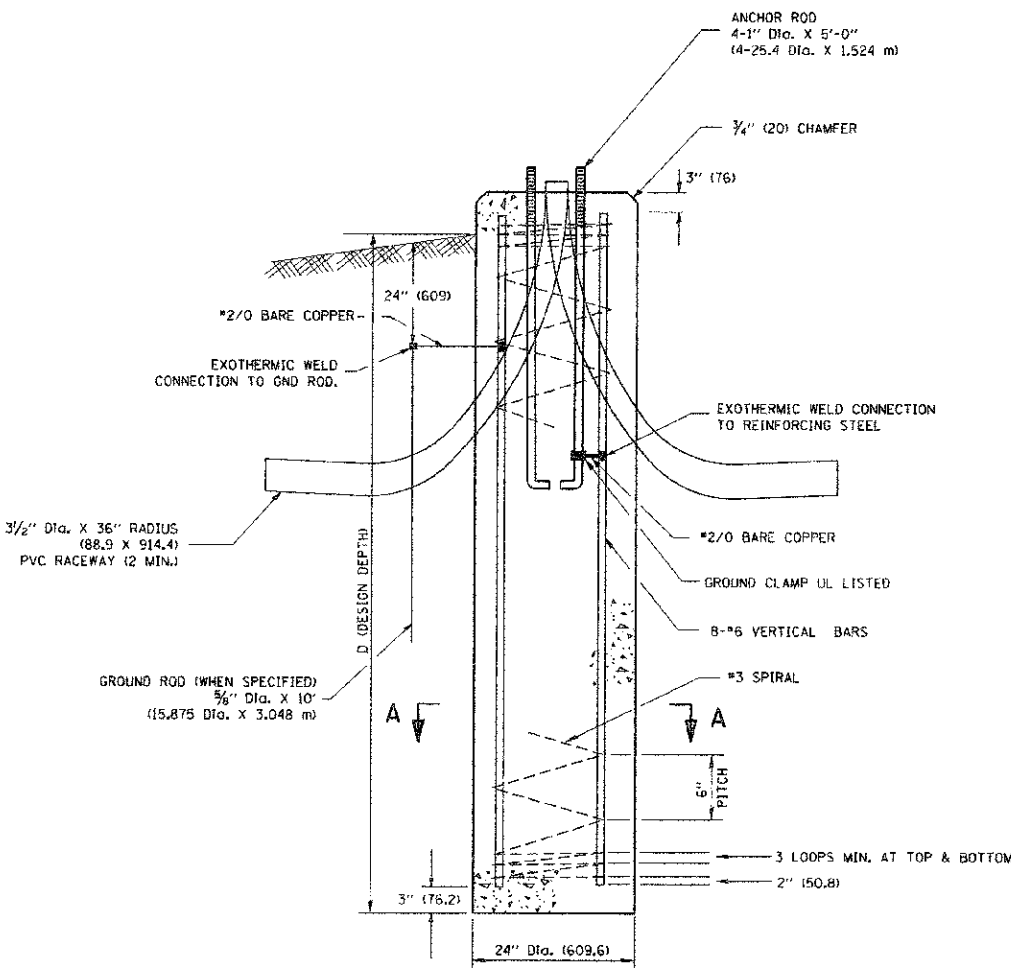
FOUNDATION DETAIL
