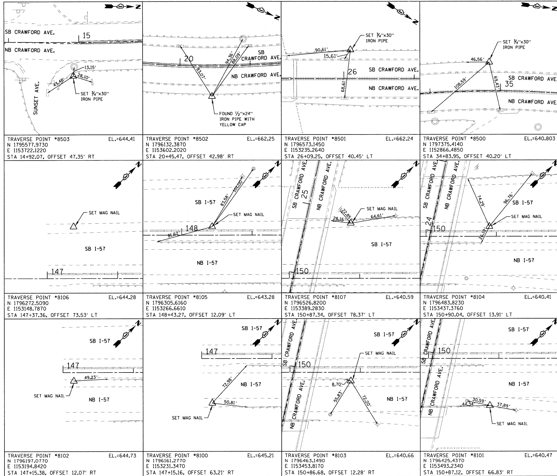
TRAVERSE CONTROL POINTS NOT TO SCALE
