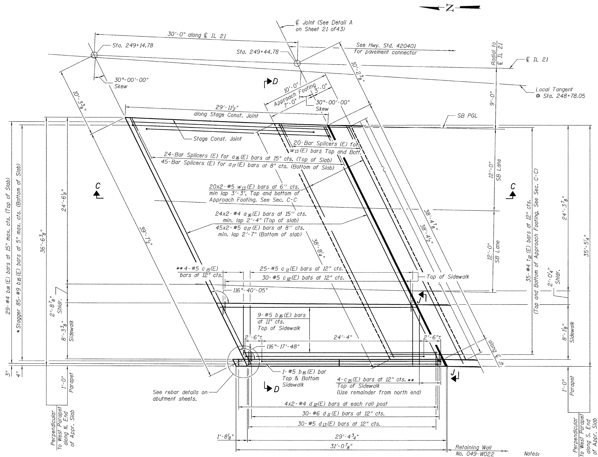
STAGE I SOUTH APPROACH SLAB PLAN
