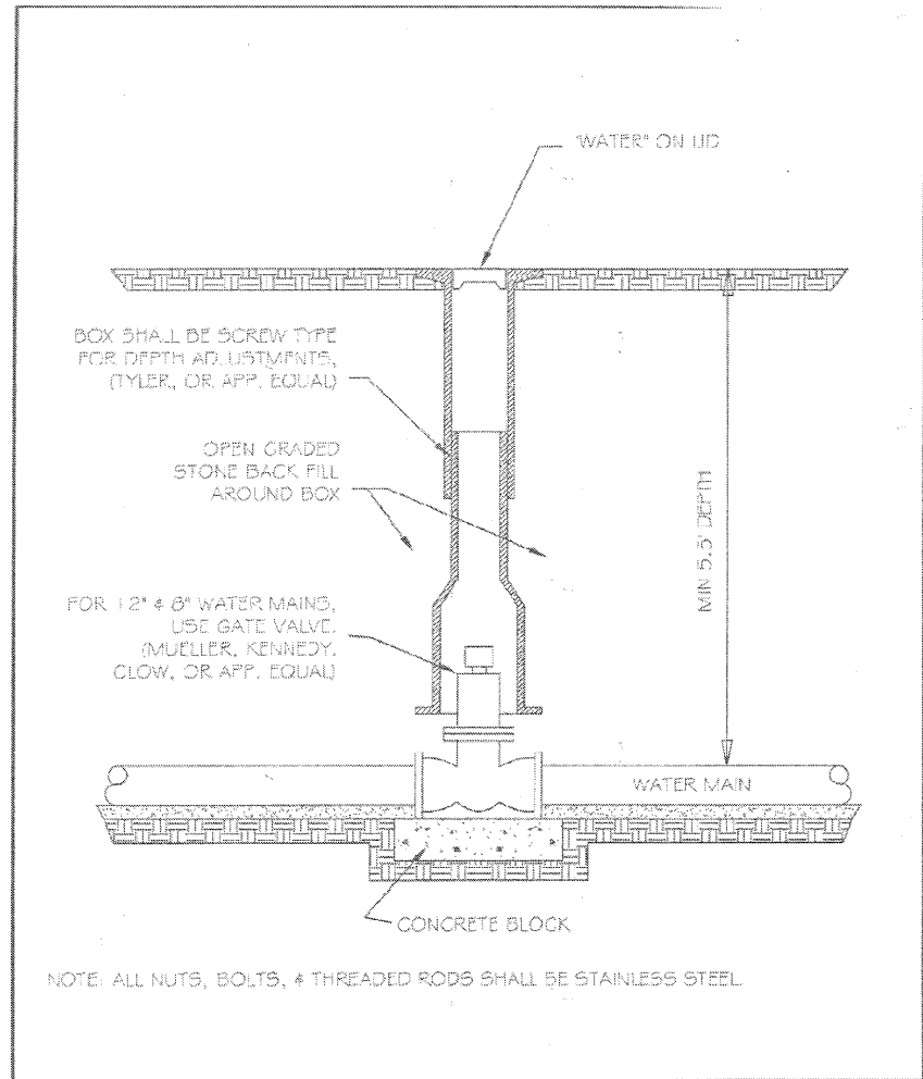
TYPICAL VALVE BOX EXHIBIT III-C-5
