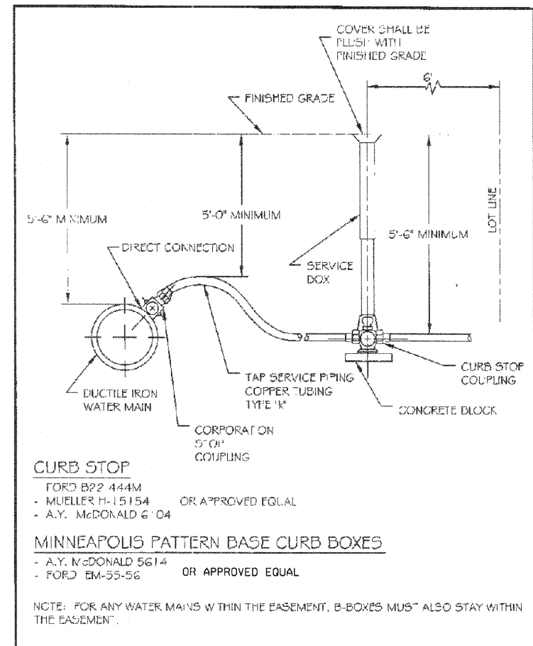
TYPICAL DOMESTIC WATER SERVICE TAP EXHIBIT III-C-6
