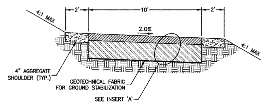
PROPOSED TRAIL TYPICAL SECTION STA. 1+00 TO STA. 18+52.79 STA. 100+00 TO STA. 103+98.74 NOT TO SCALE
