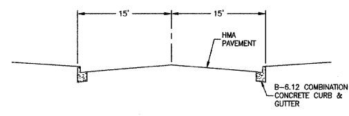
EXISTING TYPICAL SECTION PRINCEWOOD LANE NOT TO SCALE
