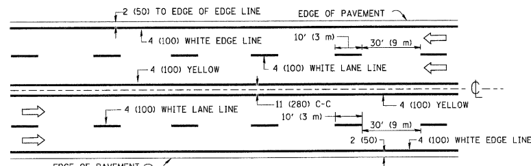
MULTI-LANE UNDIVIDED
