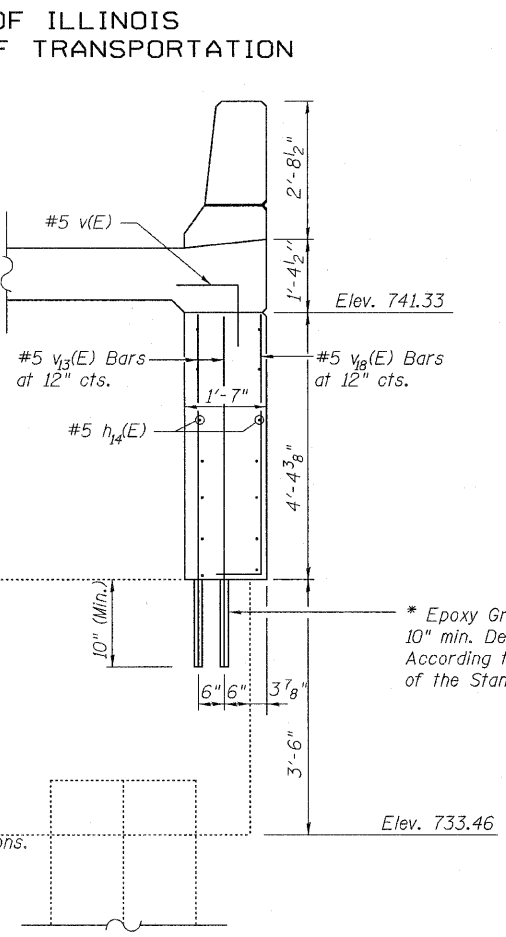
SECTION C-C
