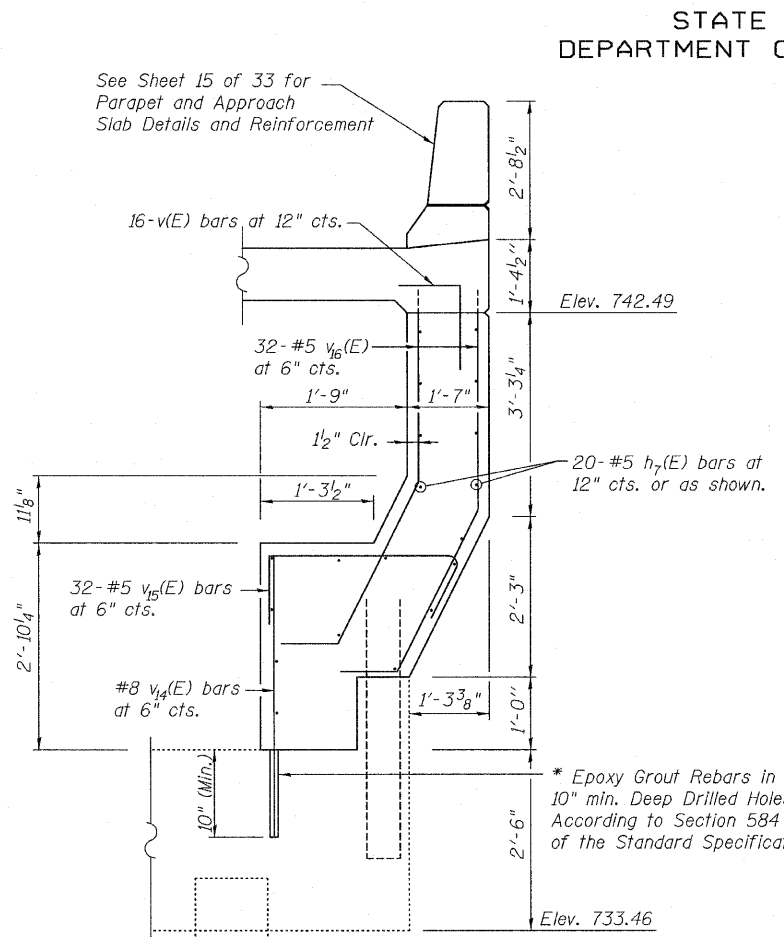
SECTION B-B
