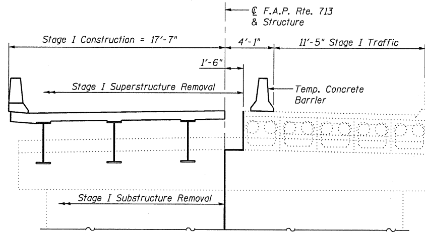
PIERS 2 & 3 - Stage I (Looking East)
