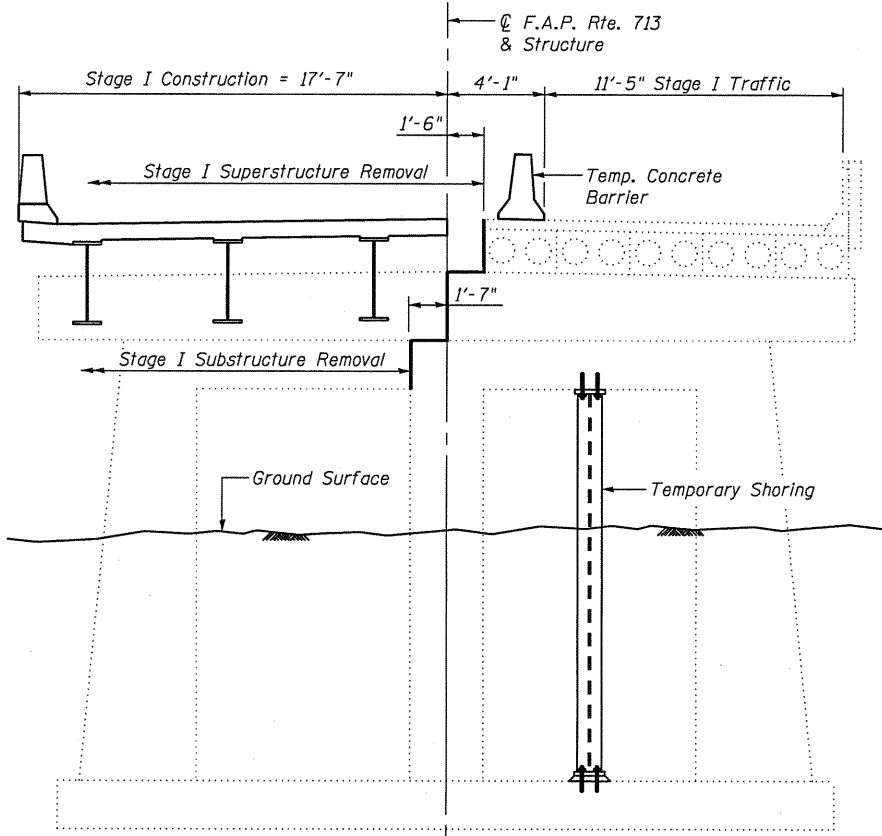
PIERS 5, 8, 9 & 10 - Stage I (Looking East)
