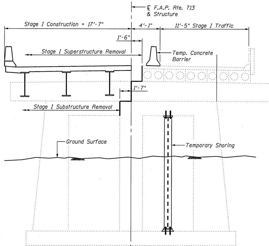
PIERS 6 & 7 - Stage I (Looking East)
