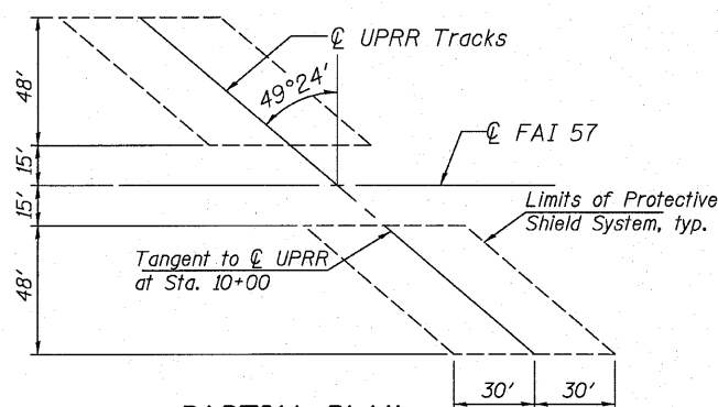
PARTIAL PLAN Showing area to be protected by Protective Shield System
